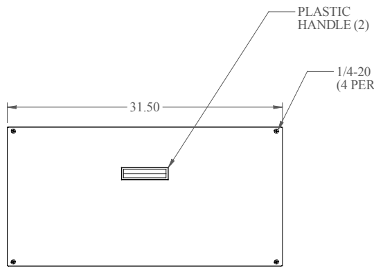
L.S. VIEW
